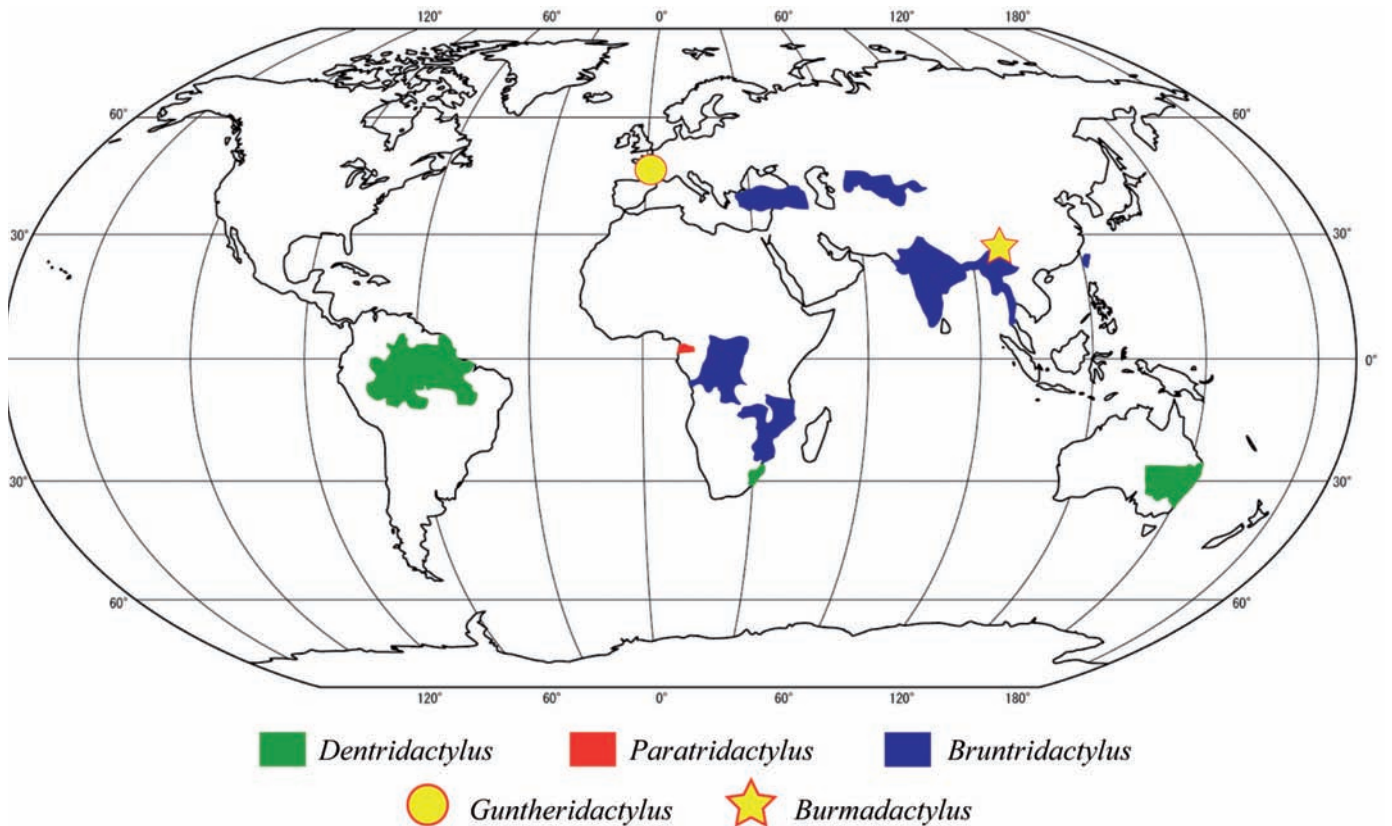
Fig. 5: Geographical distribution of Dentrictylineae.
