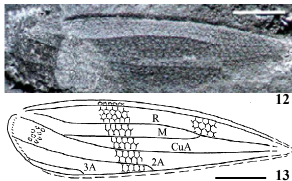
Figs 12–13. Maricoleus valentinae Shcherbakov, sp.n. (Permocupedidae), holotype PIN 5306/41, elytron: 12 — combined photographs of negative (base) and positive impression (distal part, mirrored); 13 — venation. Scale bar 1 mm.
