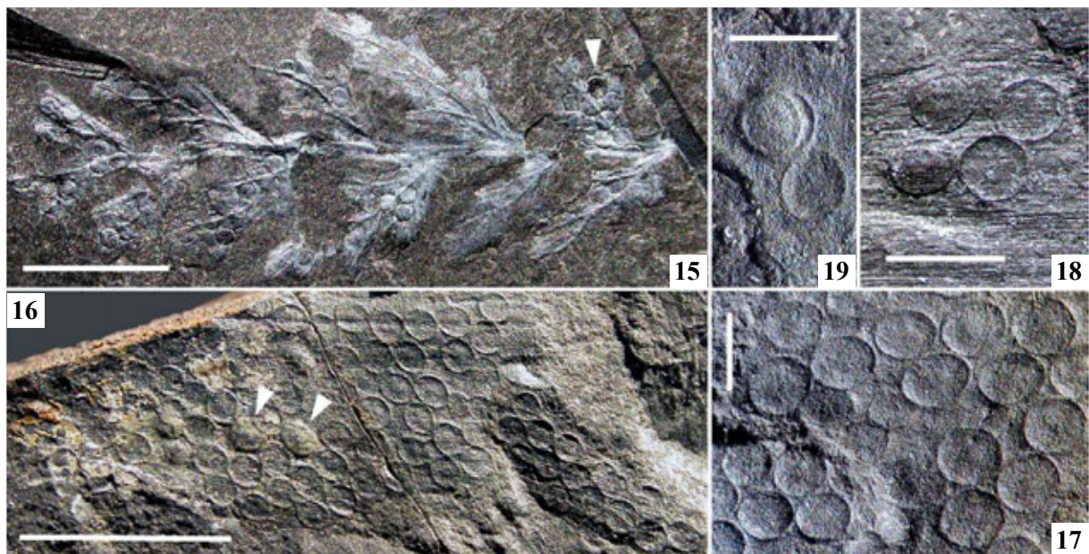
Figs 15–19. Exophytic insect eggs (?Megasecoptera) on plants: 15 — a pinna of Sphenopteris sp. with groups of empty eggshells on the upper surface of pinnules, specimen PIN 5306/84 (arrow — egg with displaced top); 16–17 — a large clutch of empty eggshells on a ?cordaite leaf fragment, specimen PIN 5306/86: 16 — entire impression (arrows: intact eggs), 17 — same, detail; 18 — two intact eggs (on the left) and two empty eggshells on a plant fragment with parallel venation, specimen PIN 5306/87; 19 — an egg with a displaced top (upper) and an empty eggshell on a pinnule of Sphenopteris sp., specimen PIN 5306/85. Scale bar 5 mm (Figs 15–16) and 1 mm (Figs 17–19).
