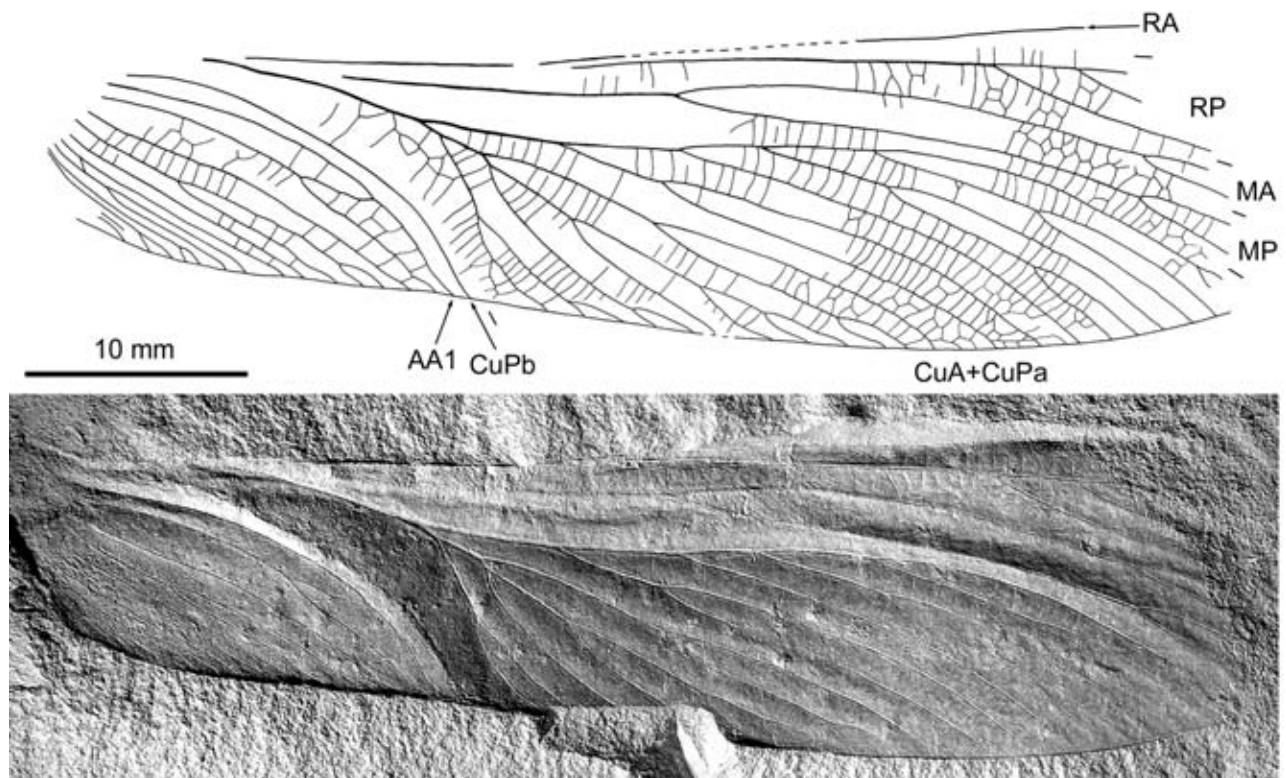
Fig. 6. Nectoptilus mazonus gen. and sp. nov. (holotype specimen FMNH PE 31978): drawing and photograph (right forewing; negative imprint, light-mirrored, reversed).
