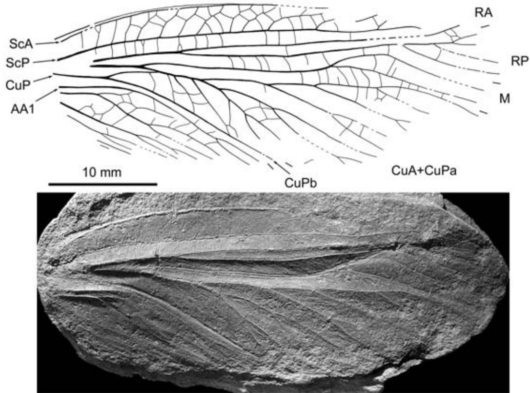
Fig. 1. Lobeatta schneideri gen. and sp. nov. (holotype specimen ROM 45568): drawing and photograph (right forewing, positive imprint, see text for vein nomenclature).
