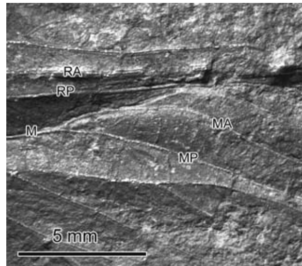
Fig. 3. Lobeatta schneideri gen. and sp. nov. (holotype specimen ROM 45568): detail of the area between RP and MP, photograph (right forewing, positive imprint, composite).
