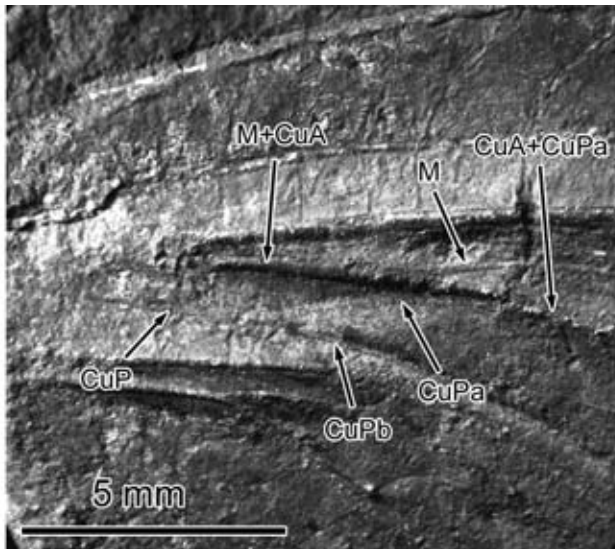
Fig. 2. Lobeatta schneideri gen. and sp. nov. (holotype specimen ROM 45568): detail of the wing base, photograph (right forewing, positive imprint, composite).
