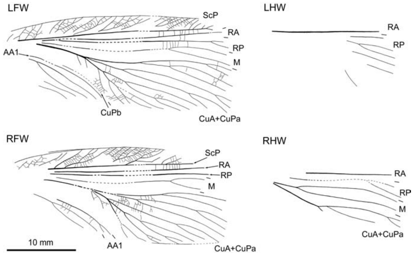
Fig. 5. Anegetus cubitalis Handlirsch 1911 (holotype specimen YPM 43); drawing, wings separated, left wings reversed (abbreviations as in Fig. 4 and also RHW: right hind wing; LHW: left hind wing).
